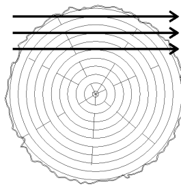
Fig. 1 Plain sawing or slicing
