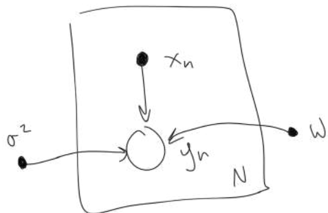
Figure 8.1: Linear regression model expressed with a DGM.
