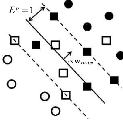
Figure 4.1: Support vectors in the soft margin perceptron.
